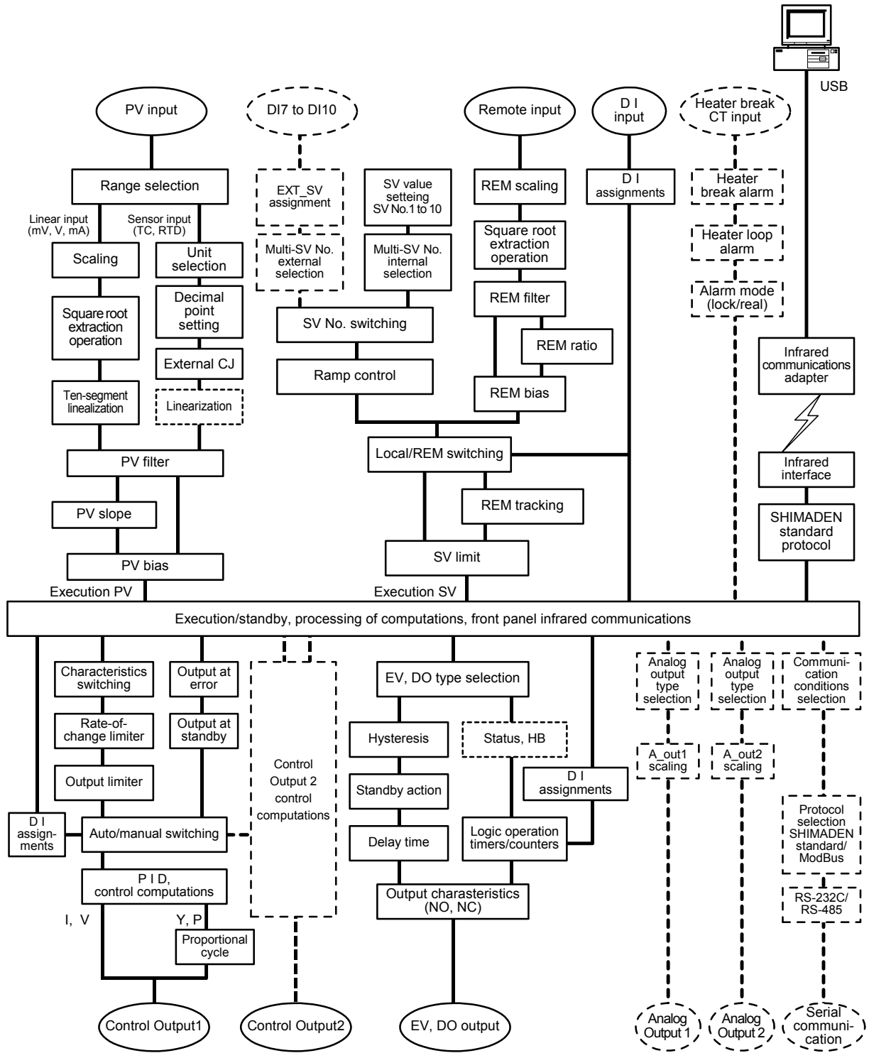
1-input Specification Function Block Diagram
