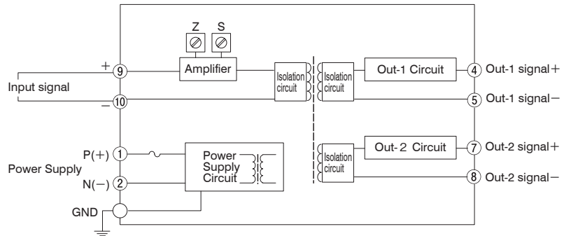
Block Diagram &amp; Terminal Wiring
