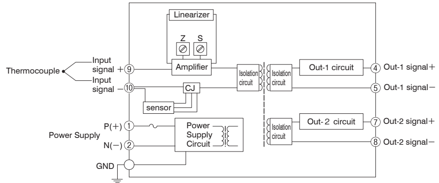
Block Diagram &amp; Terminal Wiring
