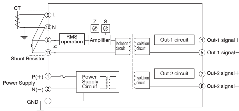
Block Diagram &amp; Terminal Wiring
