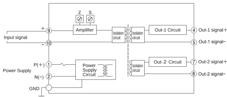
Block Diagram &amp; Terminal Wiring
