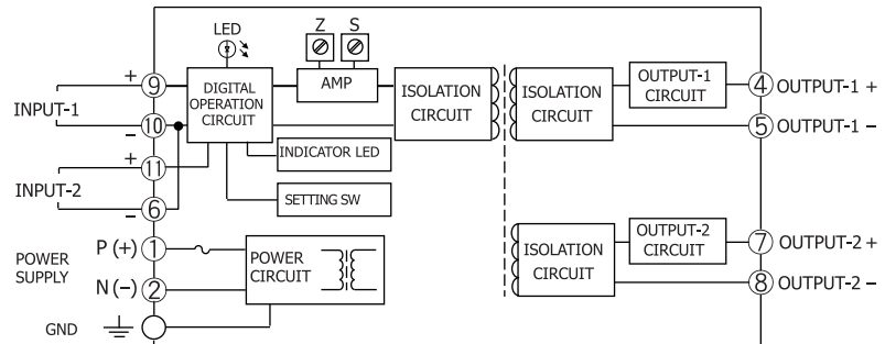
Block Diagram &amp; Terminal Wiring
