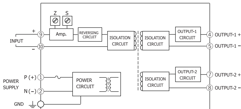
Block Diagram &amp; Terminal Wiring
