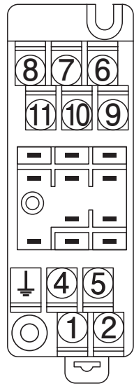
SOCKET TOP VIEW
